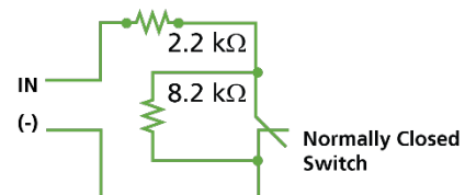
Figure 7: Normally Closed Supervised Input with Double Resistors
