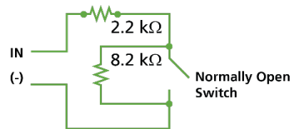
Figure 5: Normally Open Supervised Inputs with Double Resistor
